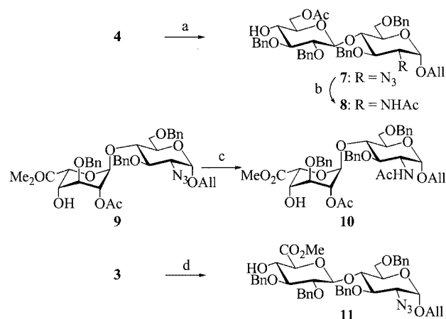
Scheme 2. Synthesis of acceptors 7 , 8 , 10 and 11 ; reagents and conditions: a) i. PPTS, MeOH, reflux, 10 min, 86%; ii. AcCl, Py, -20 °C, 90%; b) i. PPh 3 , THF/H 2 O, 9:1, 16 h. r.t.; ii. Ac 2 O, MeOH, 94%; c) i. PPh 3 , THF/H 2 O, 9:1, 16 h. r.t.; ii. Ac 2 O, MeOH, 97%; d) TFA, CH 2 Cl 2 , 15 min, 96%
