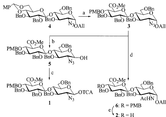
Scheme 1. Reagents and conditions: a: i. \text{PhBCl}_2 , \text{Et}_3\text{SiH} , 4 Å MS, \text{Et}_2\text{O} , -40^\circ\text{C} , 97%; ii. (\text{COCl})_2 , DMSO, \text{CH}_2\text{Cl}_2 , -78^\circ\text{C} and then \text{Et}_3\text{N} ; iii. \text{Na}_2\text{HPO}_4 , \text{NaClO}_2 , t BuOH/ \text{H}_2\text{O} , \beta -isoamylene, -10^\circ\text{C} to r.t.; iv. \text{Cs}_2\text{CO}_3 , MeI, DMF, 76%; b: i. \text{C}_8\text{H}_{14}(\text{Me}_2\text{Ph})_2\text{Ir}^+\text{PF}_6^- , \text{H}_2 , THF, r.t.; ii. \text{HgO}/\text{HgCl}_2 , acetone/ \text{H}_2\text{O} , 9:1, 83% two steps; c: \text{Cl}_3\text{CCN} , DBU, \text{CH}_2\text{Cl}_2 , 15 min 88%; d: \text{PPh}_3 , THF/ \text{H}_2\text{O} , 9:1, 16 h, r.t.; ii. \text{Ac}_2\text{O} , Pyridine, 83%; e: TFA, \text{CH}_2\text{Cl}_2 , 15 min, 94%
