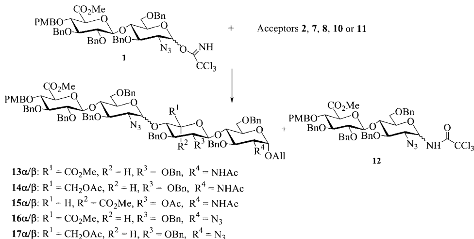
Scheme 3. Couplings reactions of donor 1 with acceptors 2 , 7 , 8 , 10 and 11 ; for reagents, conditions and α/β ratio see Table 1
