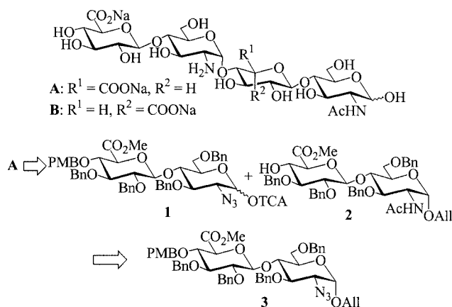
Figure 1. Retrosynthetic strategy for the preparation of GlcUA-containing HS fragments with an N -acetyl glucosamine at the reducing end
